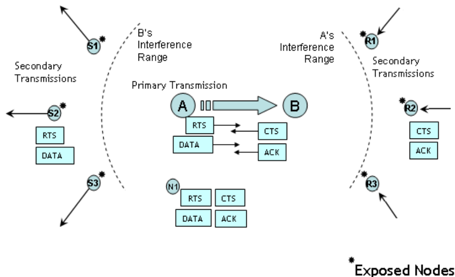
Figure 3.2: Exposed Nodes
