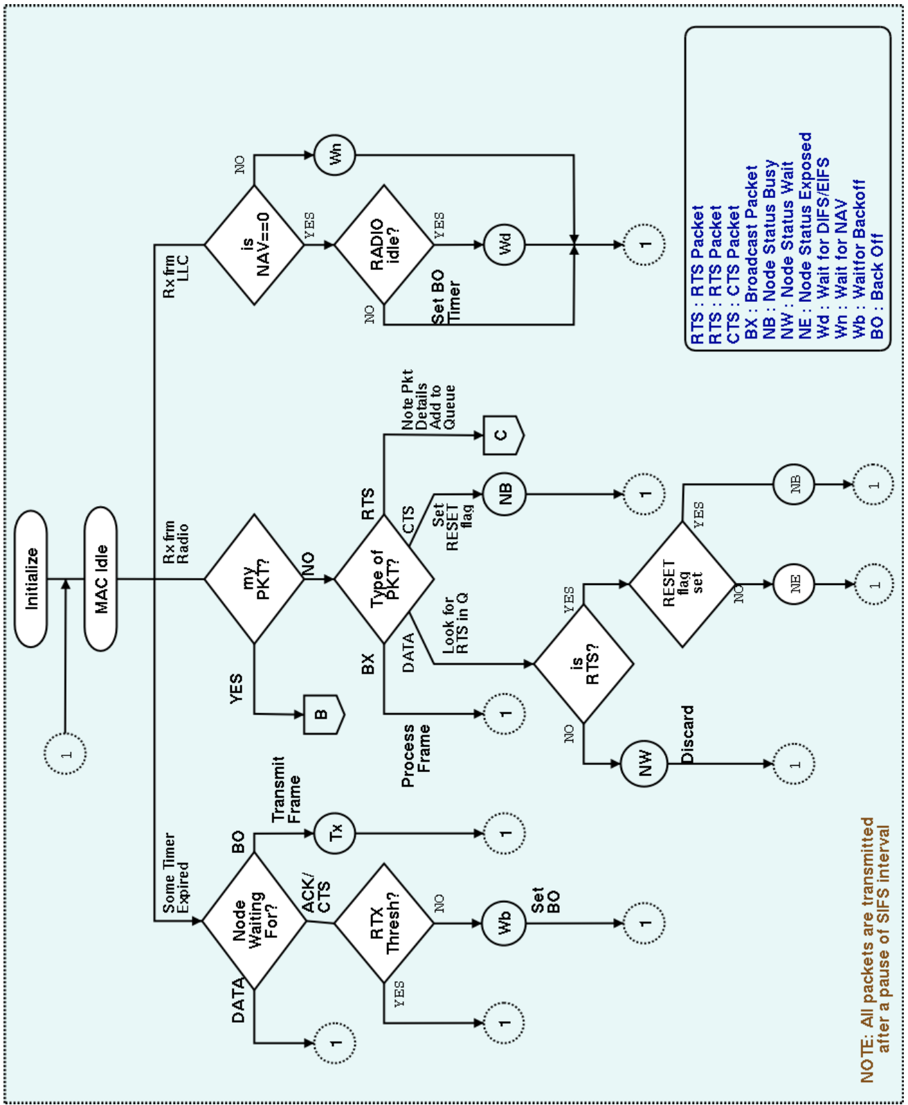
Figure 4.2: Algorithm Design
