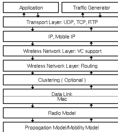
Figure 5.1: Glomosim Architecture
