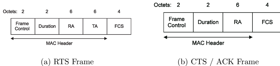
Figure 7.1: Standard 802.11 Frames
