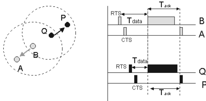
Figure 7.2: MACA-P
