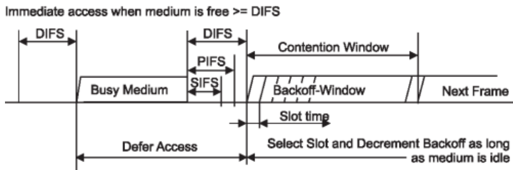
Figure 2.6: IFS Relationship
